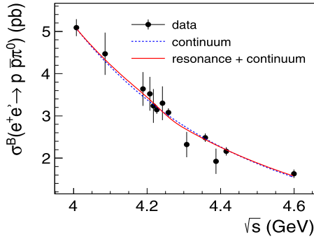
Fig. 2. Fit to \sigma(e^+e^- \rightarrow p\bar{p}\pi^0) with resonance and continuum (solid line), or only continuum term (dashed line). Dots with error bars are the measured Born cross sections. The uncertainties are statistical only.
